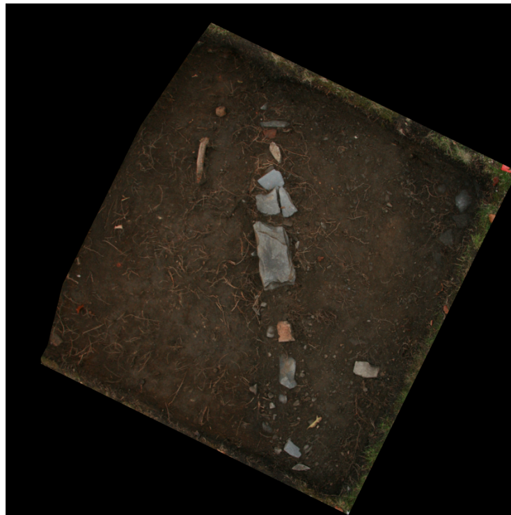
Figure 9: Completed Orthonormal Photo of Unit 13 Exported by PhotoModeler
